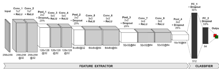
Fig. 2. Proposed CNN architecture.
