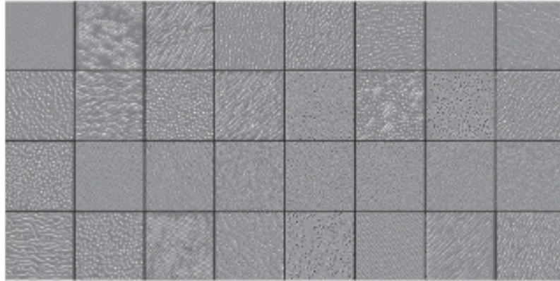
Fig. 4. Textures maximizing activations for Conv_3 layer.
